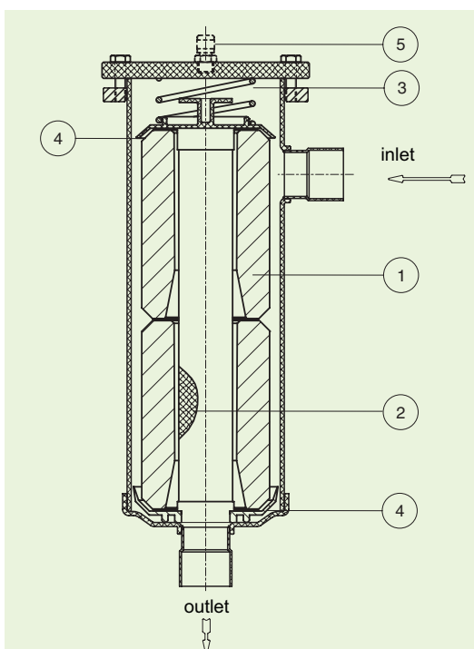
Sketch of filter with 2 blocks
