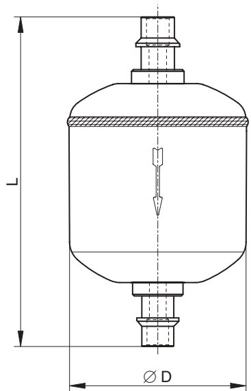
solder connections
