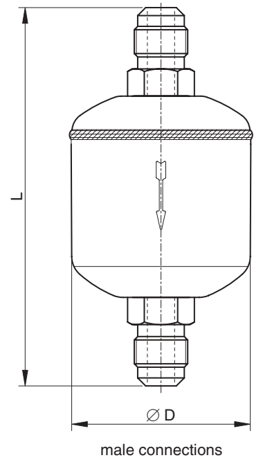
male connections
